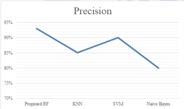
Figure 4: Precision
