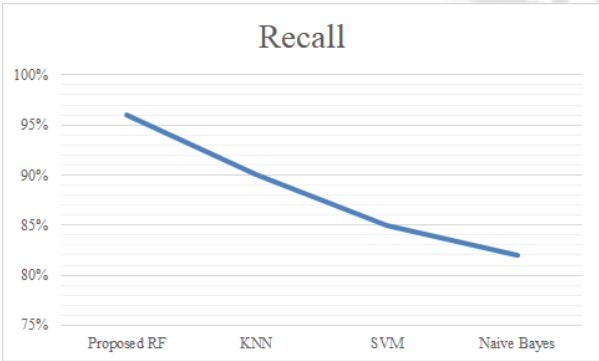
Figure 5: Recall
