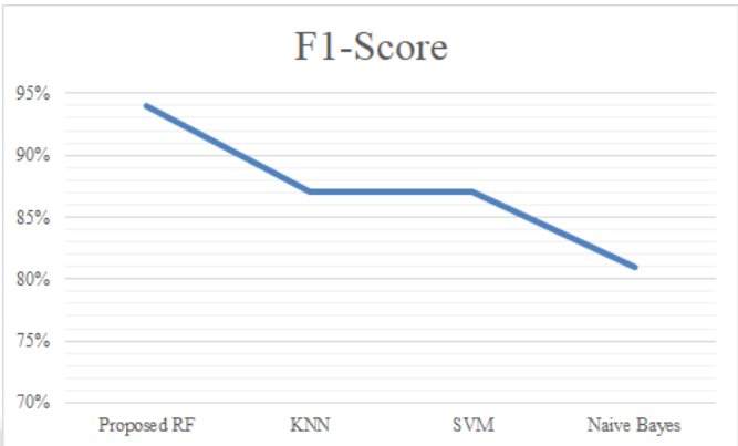
Figure 6: F1-Score
