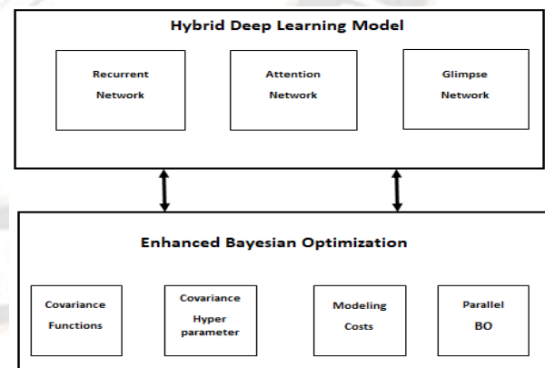
Figure 1: Proposed framework with enhanced BO for long document classification
