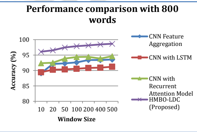
Figure 7: Performance comparison of against window size when number of words is 800
