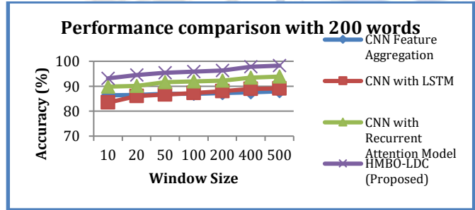
Figure 4: Performance comparison of against window size when number of words is 200 As presented in Figure 4, different deep learning models including the proposed model HMBO-LDC are evaluated for their performance in long document classification. Empirical study is made with different window size and number of words 200. Observations are made in terms of accuracy in classification. The predictions made by the models and ground truth values are used as per confusion matrix to arrive at accuracy details. Each model has shown different level of accuracy. When window size is 500, CNN feature aggregation showed 87.95% accuracy, CNN with LSTM model exhibited 89.11% accuracy, CNN with recurrent attention model showed 93.87% while the proposed model achieved 98.25% accuracy. From the results it is observed that the proposed model outperformed existing ones with highest accuracy.
