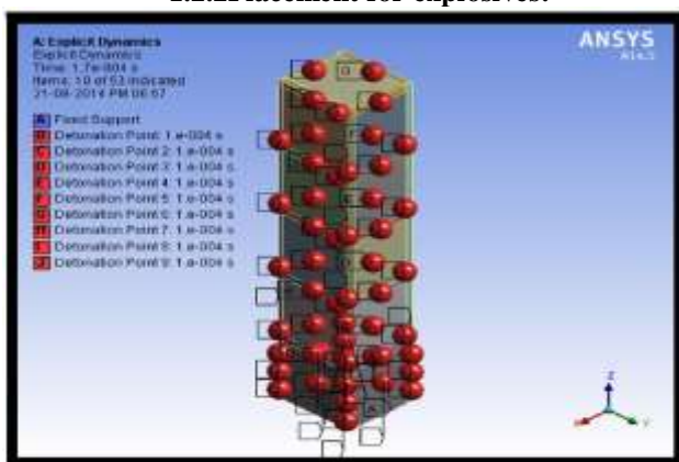
Fig.3 Proposed placement of explosive
