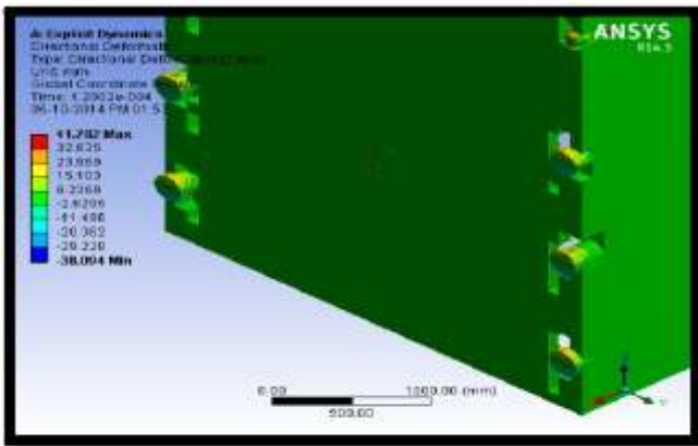
Fig.6 Directional deformation result by AUTODYNE ANSYS software For PETN explosive
