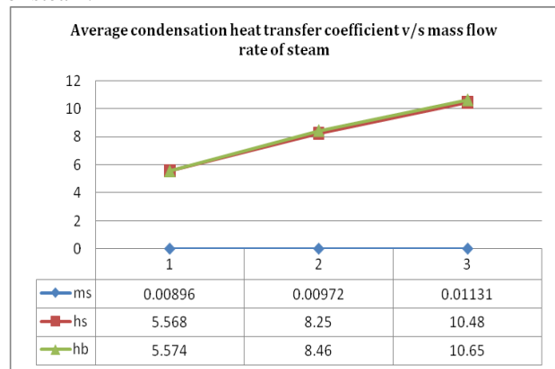
Fig.05 Plot between average condensation heat transfer coefficient v/s rates of flow of steam
