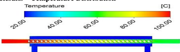
Fig.09 Temperature Distribution for Tube with simple twisted tape inserts.
