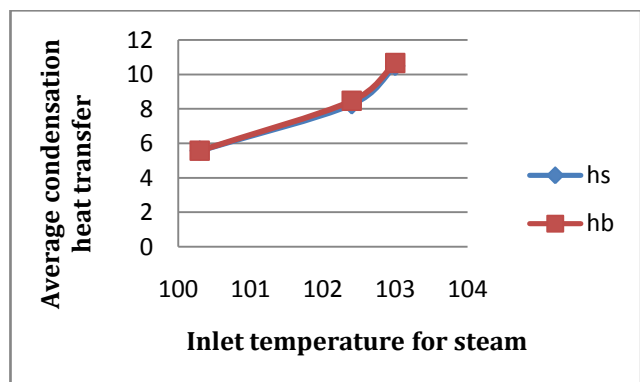
Fig.06 Plot between average condensation heat transfer coefficient v/s inlet temperatures of steam.
