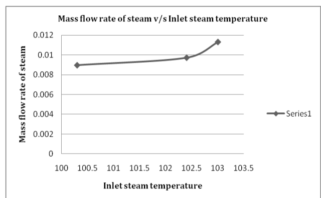
Fig.07 Plot between mass flow rate v/s inlet temperatures of steam
