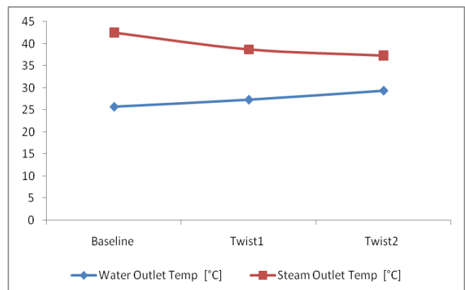
Fig.11 Variation of outlet temperatures of water and steam for simple and baffled twisted tapes.
