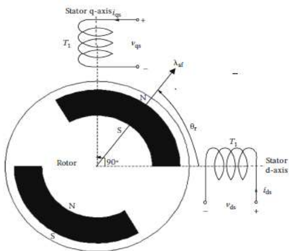
Fig.4. Dynamic model of PMSM
