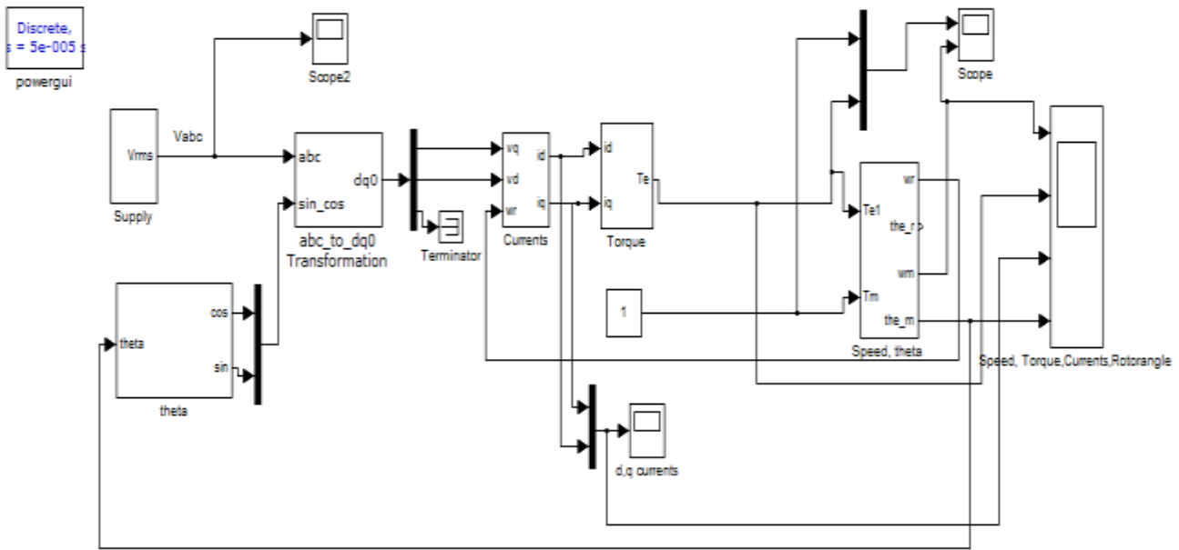
Fig 8. Simulink model of Permanent Magnet Synchronous Motor
