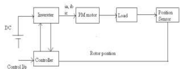
Fig.1 Block diagram of PMSM drive system
