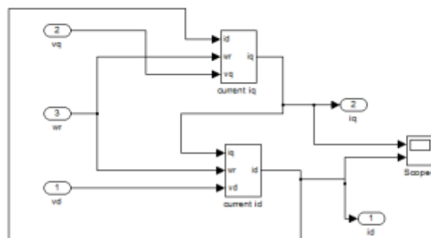
Fig.5. i_d, i_q current blocks
