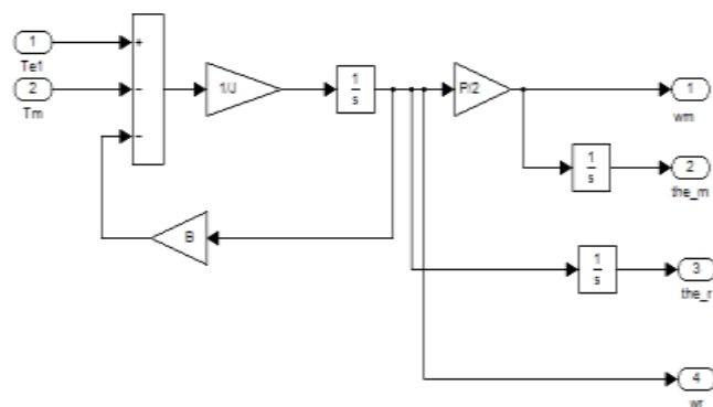
Fig.6. Speed model blocks
