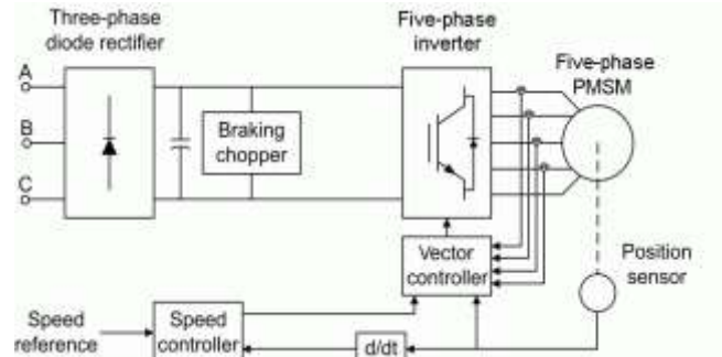
Fig 10. Proposed five phase PMSM modeled block diagram
