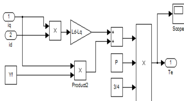
Fig.7. Torque model blocks of PMSM
