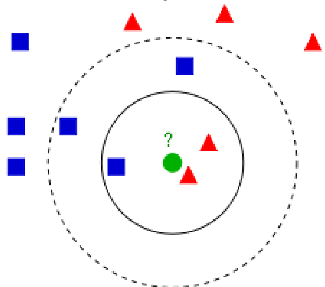
Fig.1. k-NN Classification
