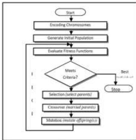
Figure 2: Genetic algorithm Process
