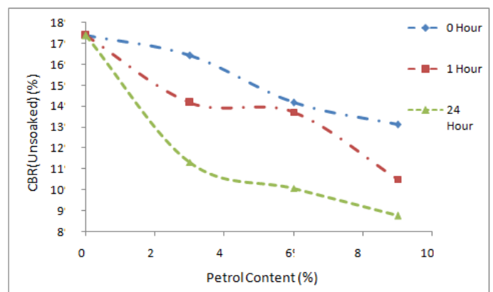
Fig 6: Effect of Petroleum Products on CBR
