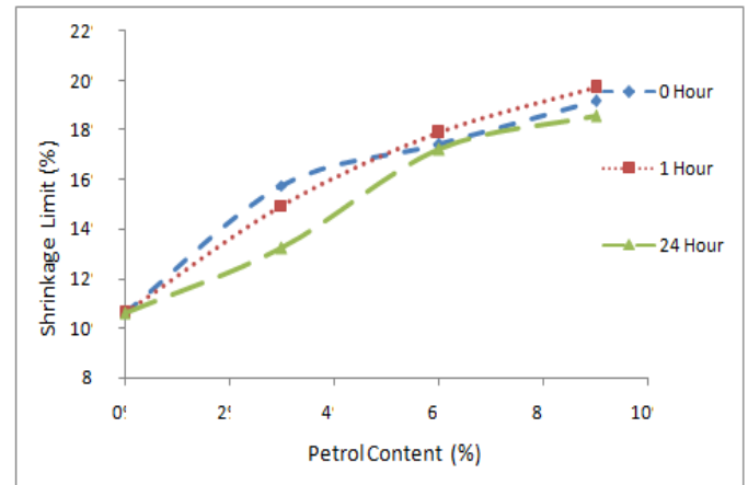
Fig 4 :Variation of Shrinkage Limit with Petrol
