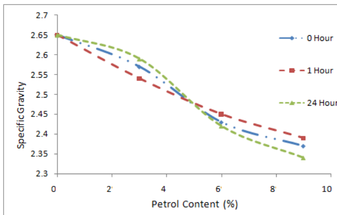
Fig 3 :Variation of Specific Gravity with Petrol
