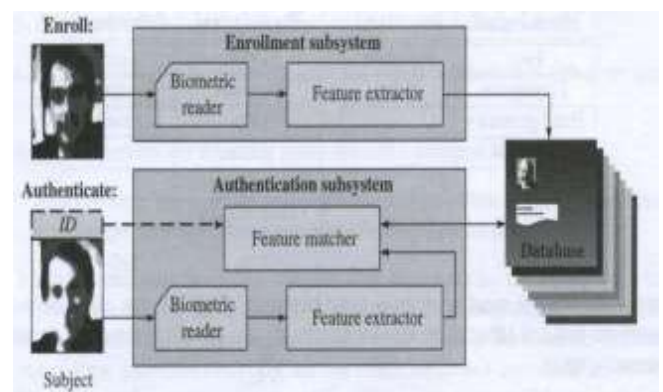
Fig 1: Typical Structure for Biometric Identification System
