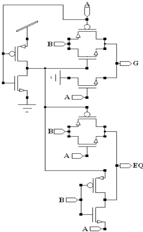
Figure 3. Schematic of Stage 0 th of Existing 64-Bit Binary Comparator
