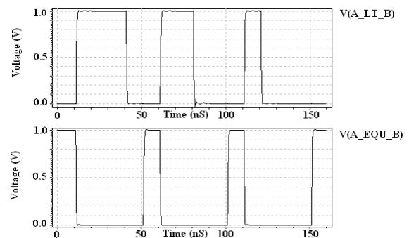
Figure 12. Waveforms of Modified 64-Bit Binary Comparator
