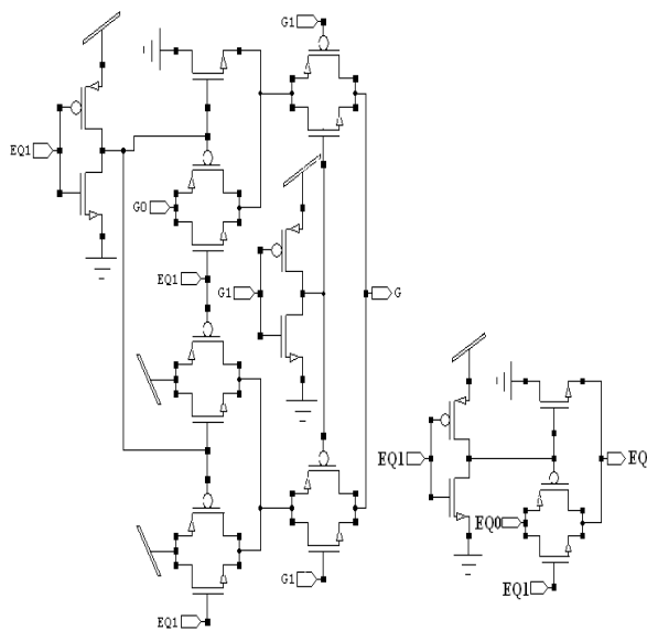
Figure 8. Schematic of Stage 1 st of Modified 64-Bit Binary Comparator
