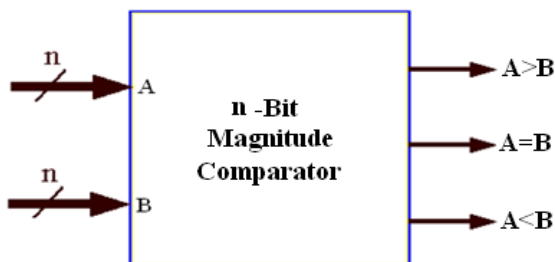
Figure 1. Block Diagram of n-Bit Magnitude Comparator
