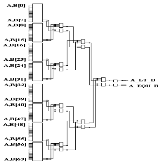
Figure 11. Schematic of Modified 64-Bit Binary Comparator
