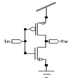
Figure 10. Schematic of Inverter of Modified 64-Bit Binary Comparator
