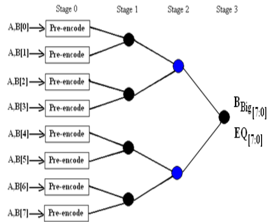
Figure 2. Tree-Diagram of 8-Bit Binary Comparator
