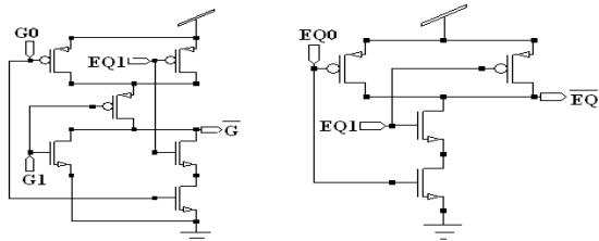
Figure 9. Schematic of Stage 2 nd of Modified 64-Bit Binary Comparator
