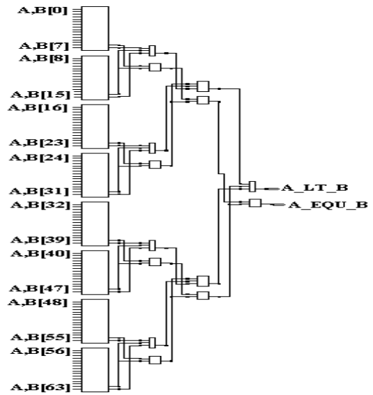
Figure 6. Schematic of Existing 64-Bit Binary Comparator
