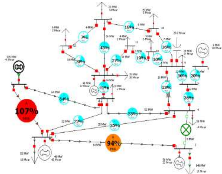
Fig. 4. Modified IEEE 14 bus in which line 1-2 is overloaded when 3-4 line is outaged
