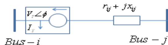
Fig.1. Equivalent circuit of TCPAR
