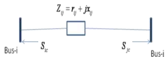
Fig. 2. Injection model of a TCPAR
