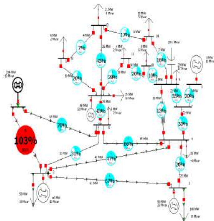
Fig. 3. Modified IEEE 14 bus system
