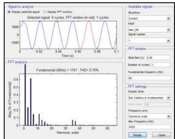
Fig.8 FFT analysis with filter of current
