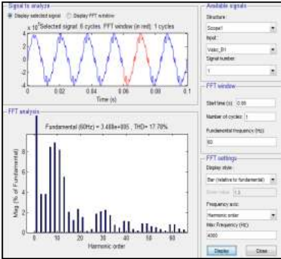
Fig.8 FFT analysis without filter of voltage
