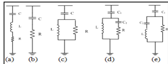
Fig. 3 (a) Single- tuned (b) 1st order high-pass (c) 2nd order high-pass (d) 3rd order high-pass (e) C-type.
