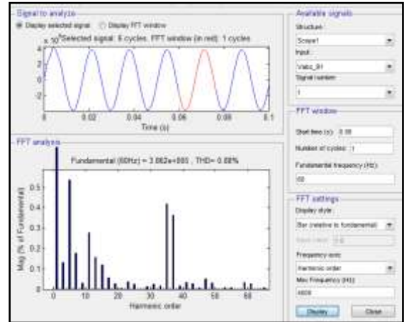
Fig.10 FFT analysis with filter of voltage
