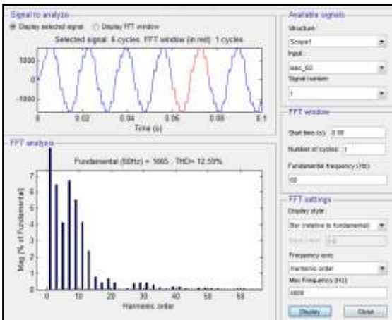
Fig.9 FFT analysis without filter of current
